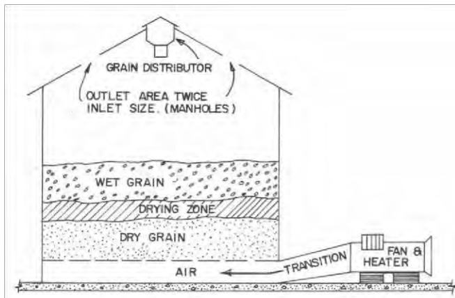
Figure 1. Grain is dried from the point of air entry with the drying front moving in the direction of air flow. The wetter grain occurs where the air leaves the grain layer.
