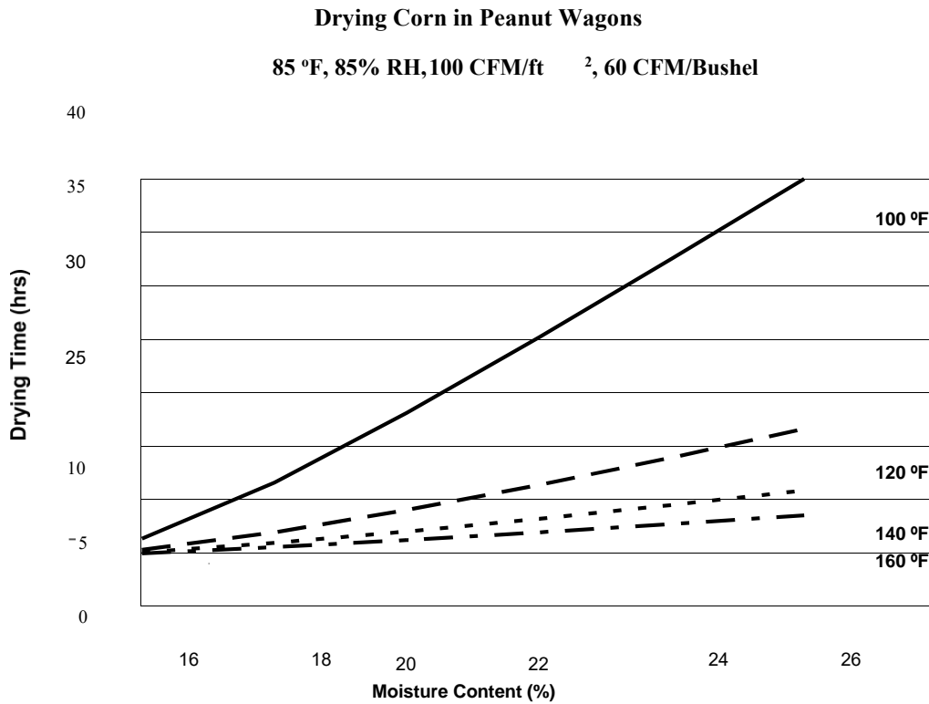
Figure 3 Estimated total drying time for corn with air at 85°F and 85 percent relative humidity, 60 CFM/Bushel, 100 CFM/ft 2 of floor area
