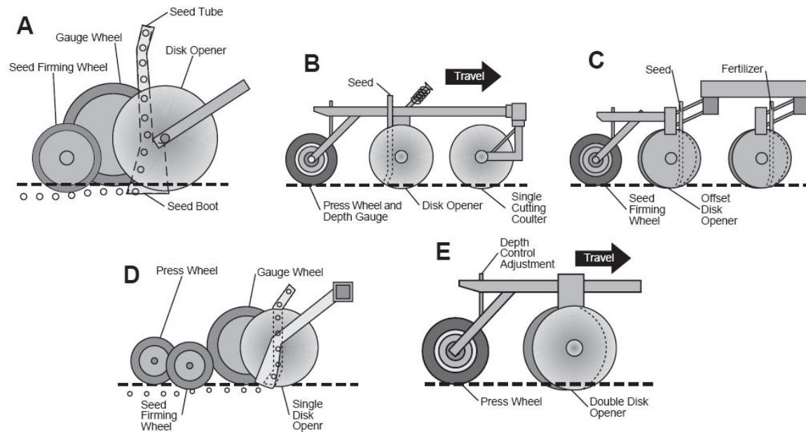
Figure 2. Diagram of typical seeding mechanisms: A) Single disk opener, B) single disk opener with add-on coulters, C) offset double disk openers with fertilizer opener mounted midway between seed openers, D) depth control is maintained by mounting the gauge wheel beside the seed opener disk, E) depth control is maintained by mounting the press wheel on the furrow opener frame member.
